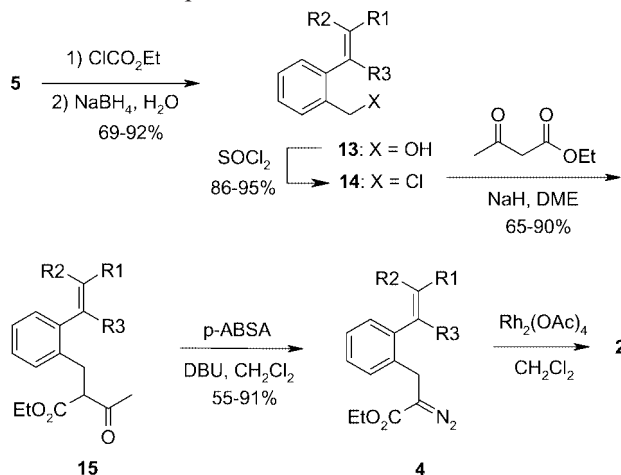
Scheme 3. An alternative route to compounds of type 2 .
